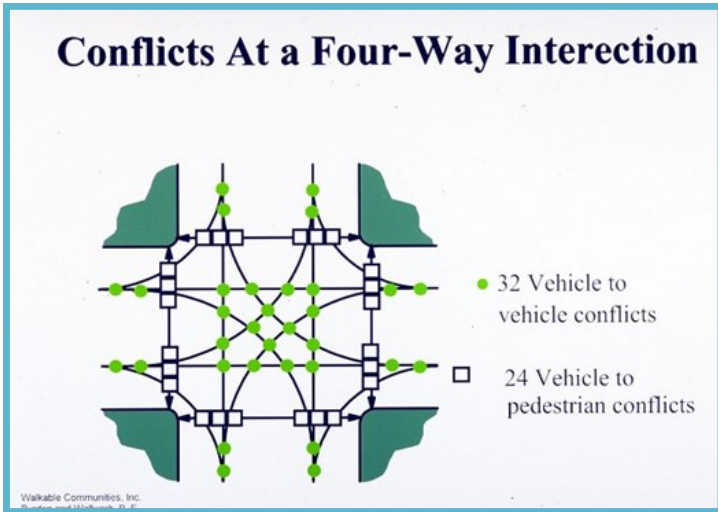
Example of the conflicts at a typical four-way intersection. (Image courtesy of Dan Burden )
