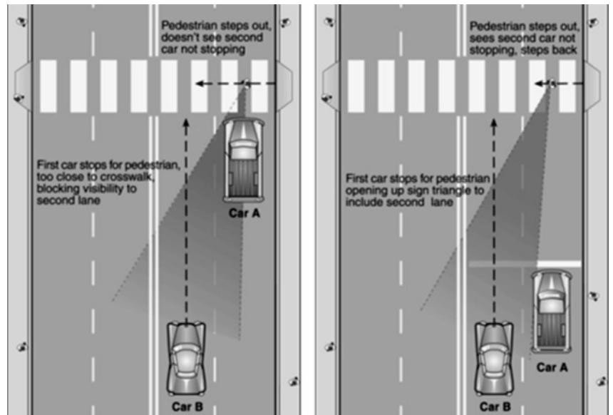
Example illustrating "multiple-threat" conflict (left) and advance stop line (right, image courtesy of FHWA)
